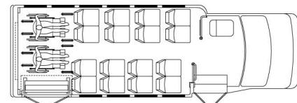
16 Passengers and 2 W/C, rear lift
