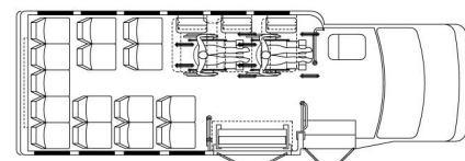
15 + 6 Passengers and 2 W/C, front lift
