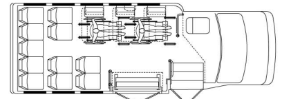
11 + 6 Passengers and 2 W/C, front lift
