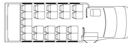
21 Passengers + 30" Rear Luggage
