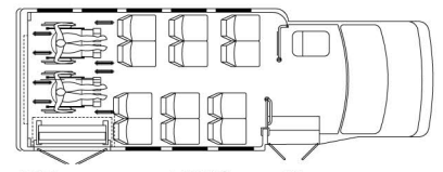
12 Passengers and 2 W/C, rear lift
