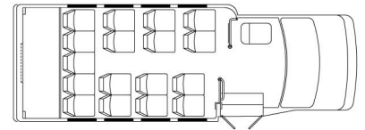
17 Passengers + 30" Rear Luggage
