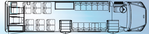
37' 24 Passenger with 2 Wheelchair Positions and Mid-Ship Door
