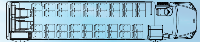
40' 36 Passenger with 2 Wheelchair Positions
