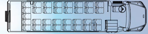
35' 33 Passenger with Rear Luggage
